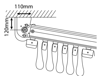
Ceiling Fixing
