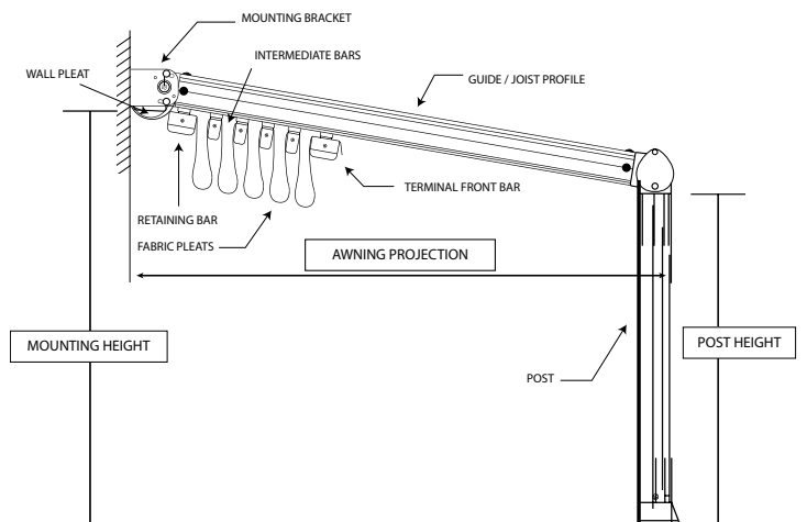
Genius A1 Awning Side View
